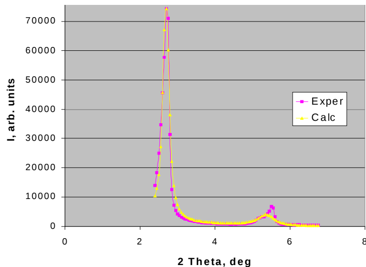
System 1: <10% single layers, the rest in stacks of 20-30 platelets each with interlayer separation \sim 3.7 nm
