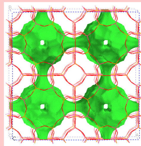
Accessible Volume ( r=1.4 \text{ \AA} )
