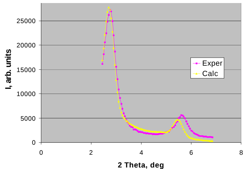
System 2: \sim 50\% single layers, the rest in stacks of 6-8 platelets each with interlayer separation \sim 3.9 nm
